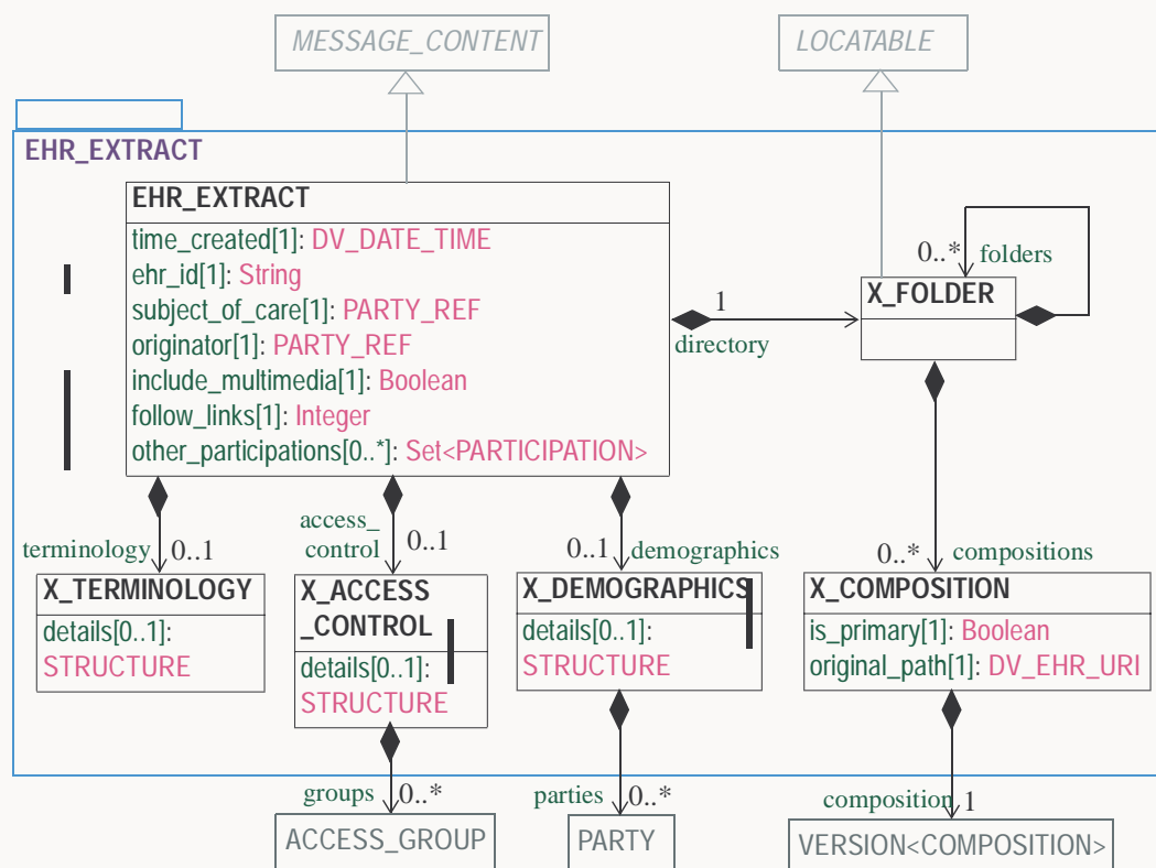
FIGURE 3 RM.EHR_EXTRACT Package
