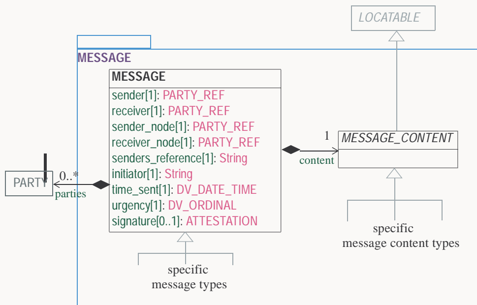
FIGURE 2 RM.MESSAGE Package
