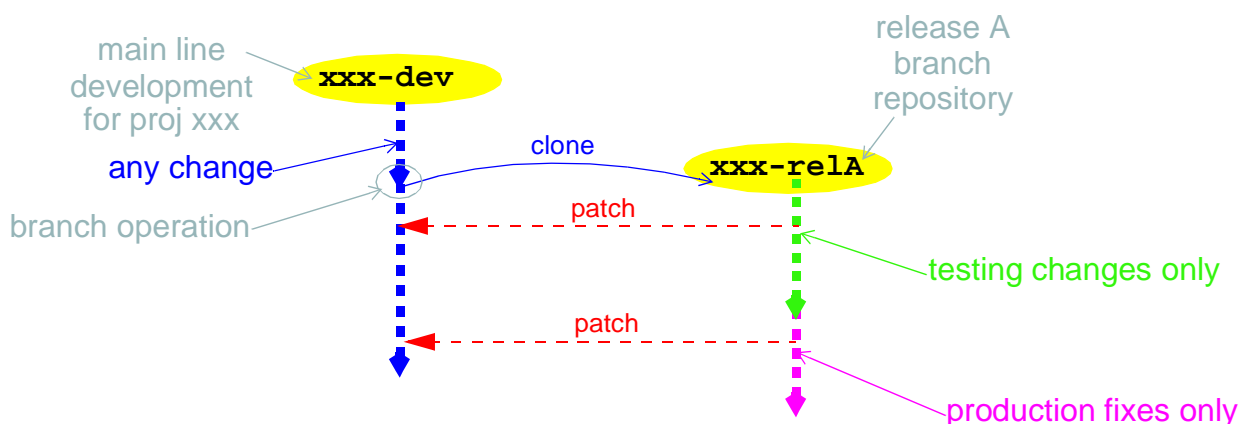
FIGURE 10 Branching
