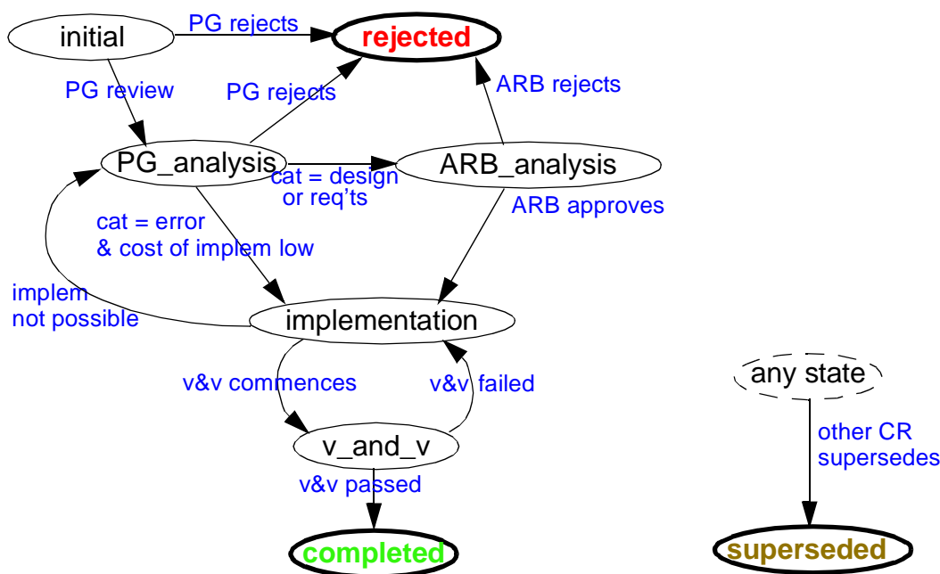
FIGURE 16 CR Lifecycle
