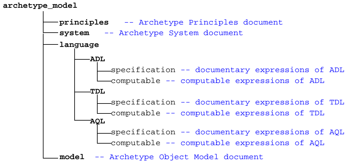
FIGURE 8 Specification Project - archetype_model directory
