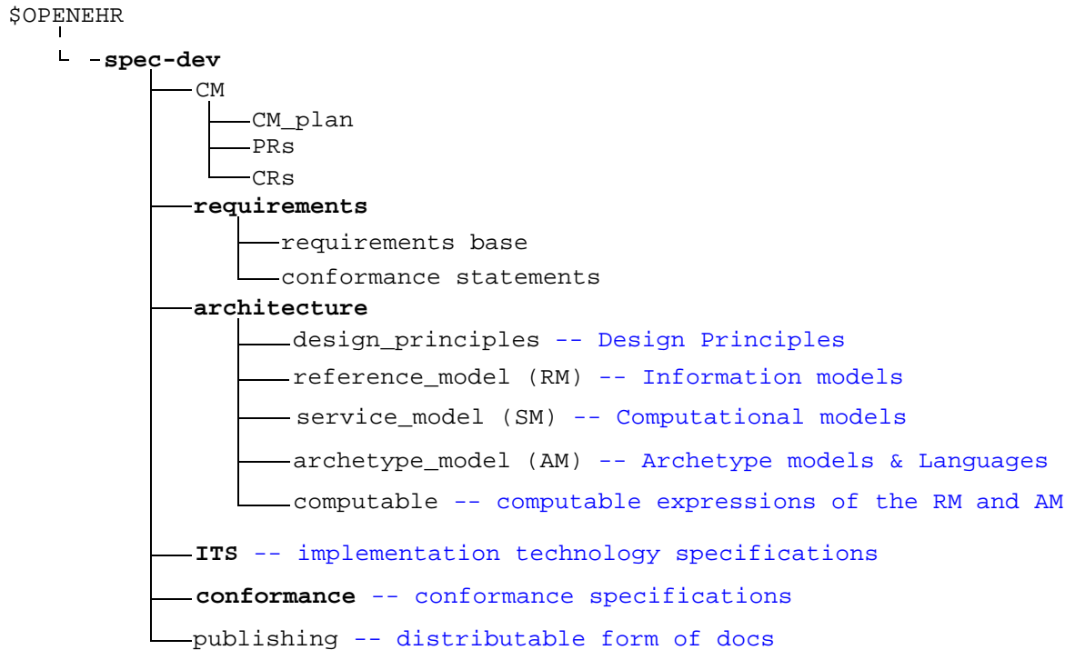
FIGURE 6 Structure of spec Repository
