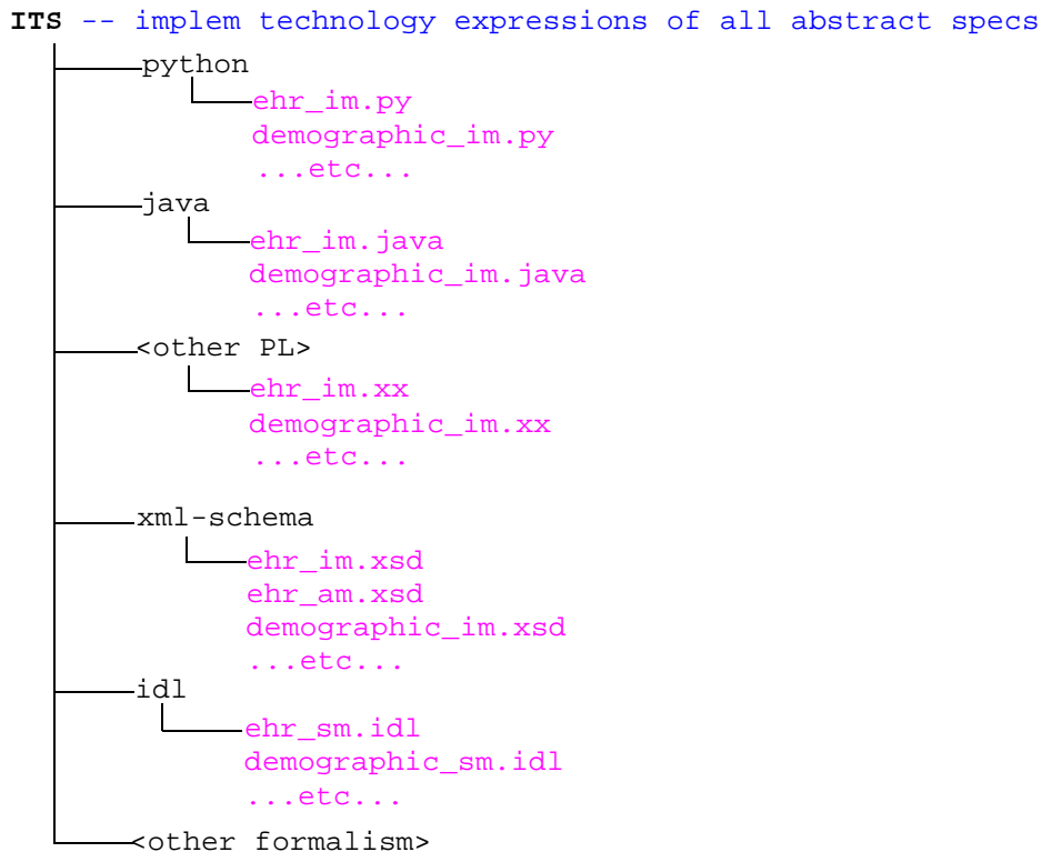
FIGURE 9 ITS Directory Structure
