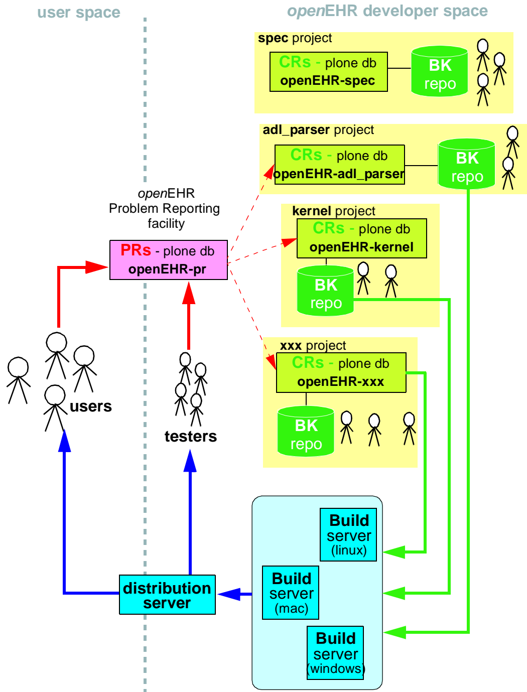
FIGURE 19 Tool Environment of openEHR projects
