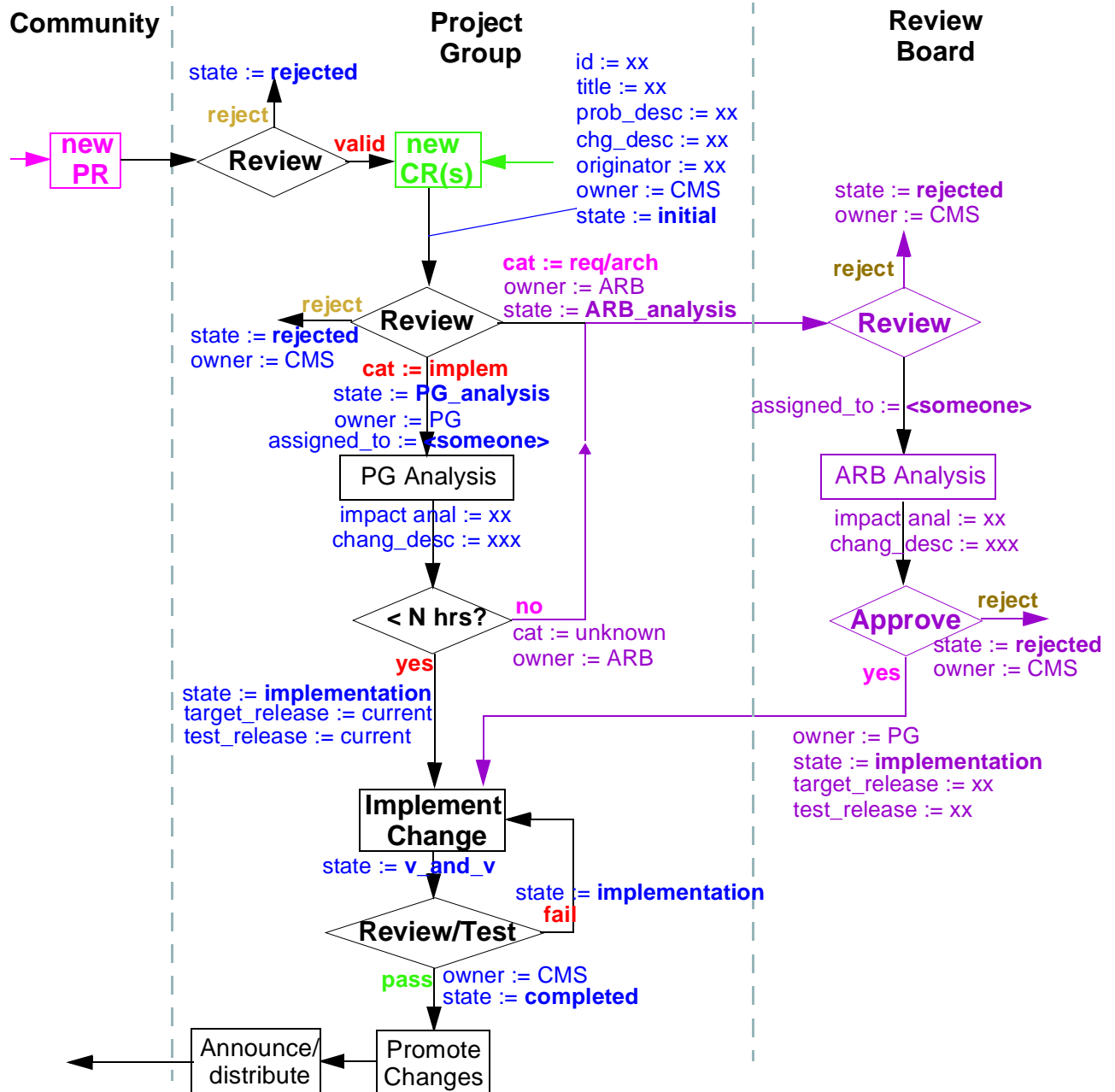
FIGURE 15 openEHR Change Request Process for reference project
