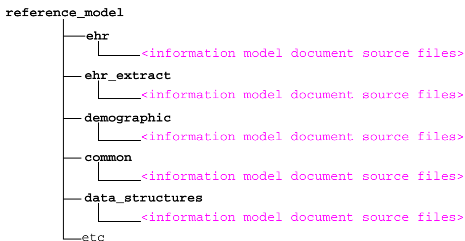
FIGURE 7 Specification Project - reference_model directory
