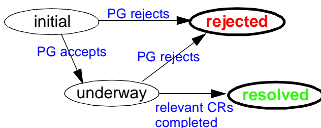
FIGURE 14 PR Lifecycle
