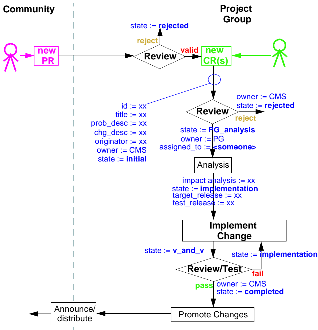
FIGURE 17 openEHR Change Request Process with no review board
