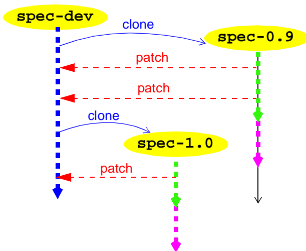
FIGURE 11 openEHR Release Structure for spec repository
