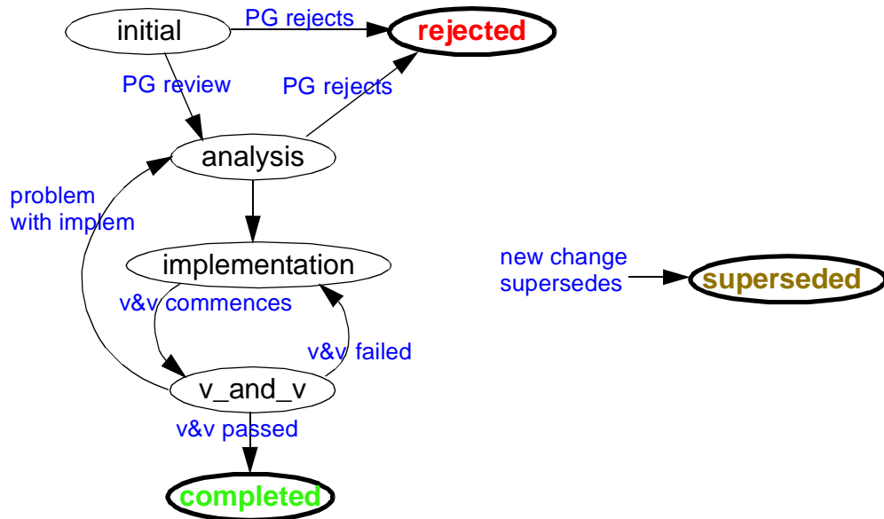
FIGURE 18 Simple CR Lifecycle
