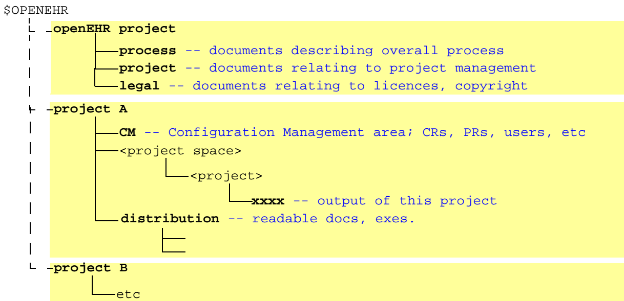
FIGURE 5 General Directory Structure of openEHR Repositories
