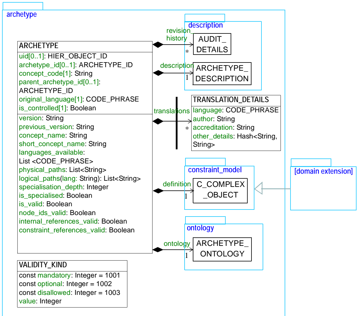
FIGURE 4 openehr.am.archetype Package
