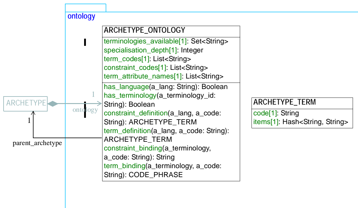
FIGURE 10 openehr.am.archetype.ontology Package
