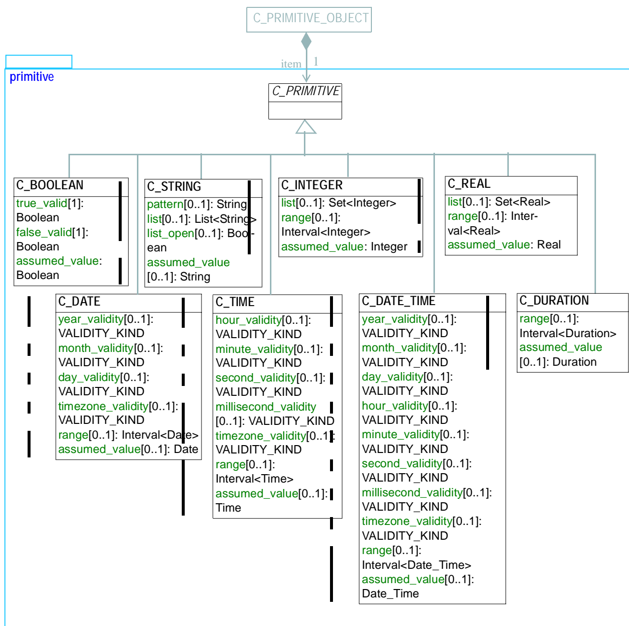
FIGURE 9 The openehr.am.archetype.primitive Package
