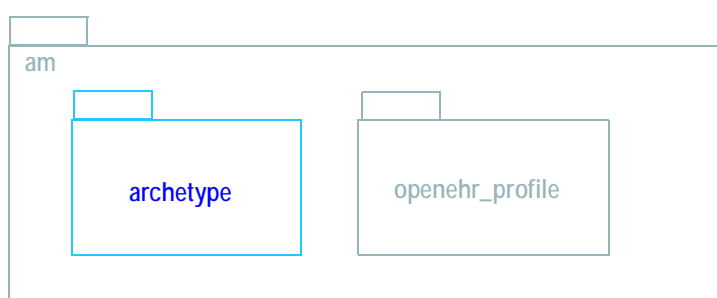
FIGURE 2 openehr.am.archetype Package
