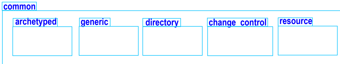
FIGURE 1 rm.common Package
