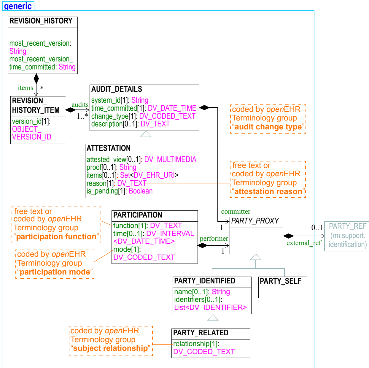
FIGURE 4 rm.common.generic Package
