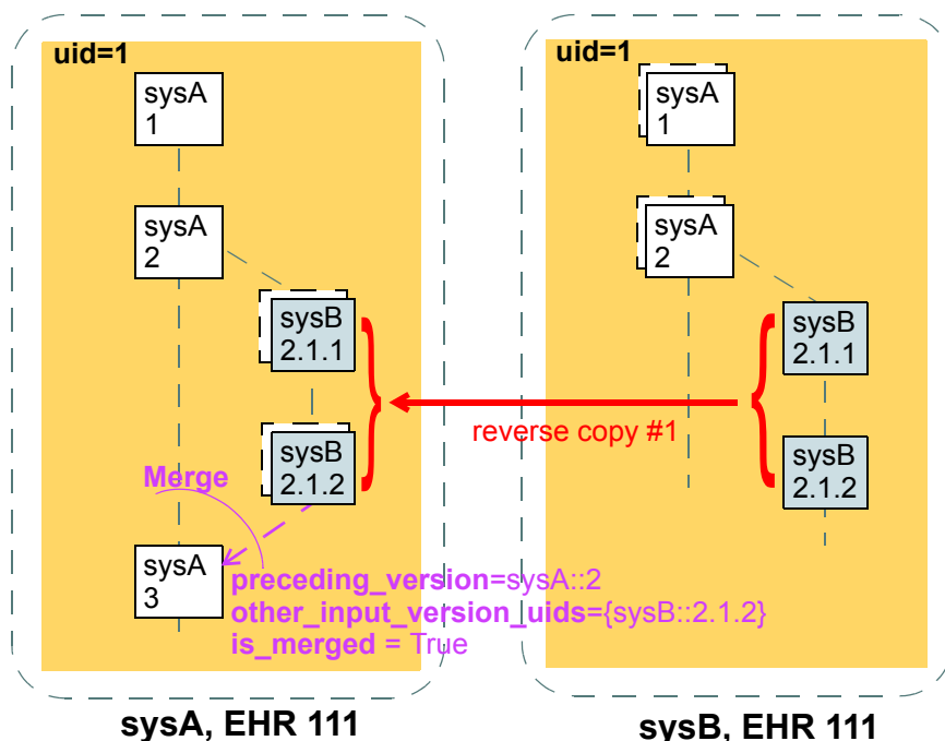
FIGURE 13 Version Merging
